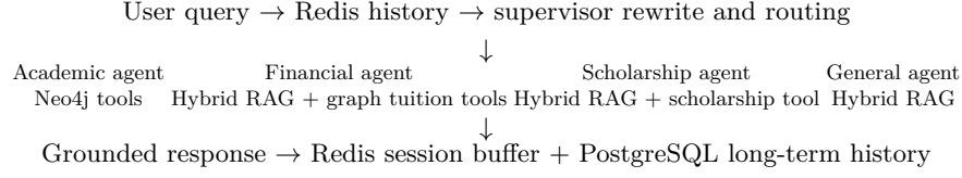
Fig. 1. CTU-Chat online orchestration path.
